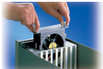
2个热插拔53-CFM 散热风扇模块
